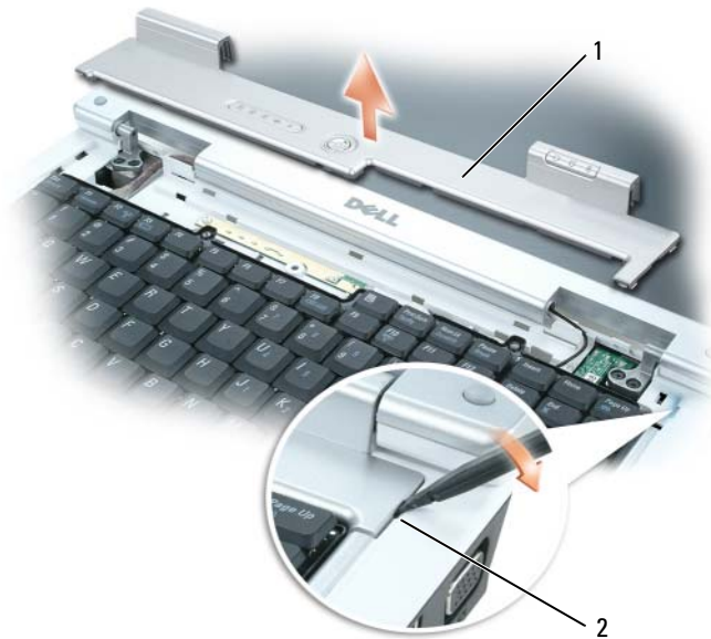
1 铰接护盖
